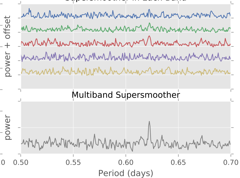
Supersmooter in Each Band
