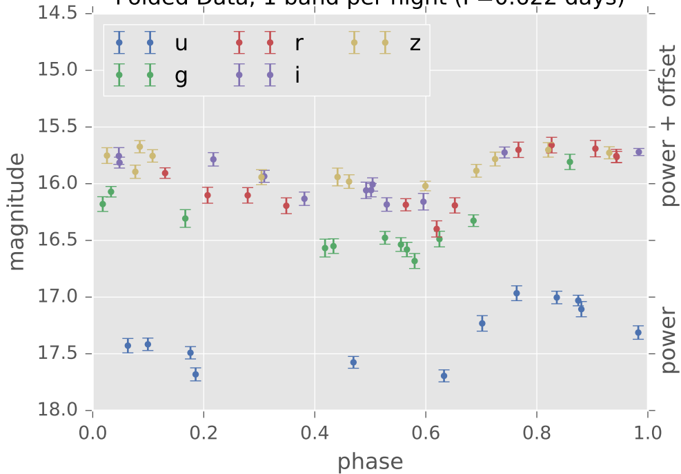
Folded Data, 1 band per night (P=0.622 days)
